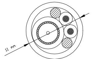
RG 59B/U + 2 x 1 mm 2
